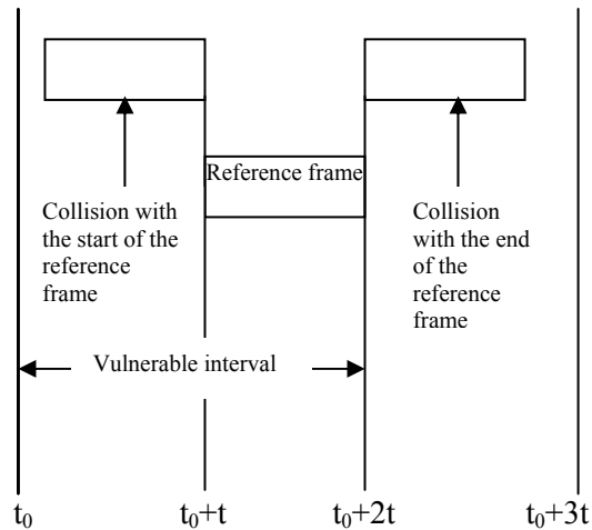
Figure 4: Vulnerable Period
