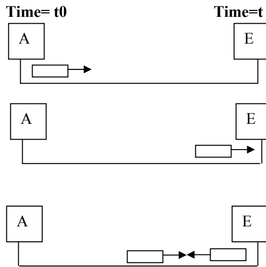
Figure 8: Collision detection
